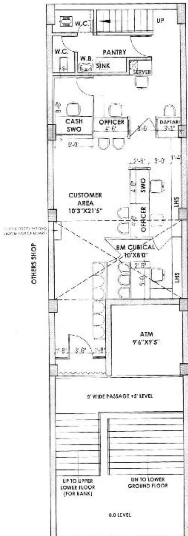
UPPER GROUND FLOOR
