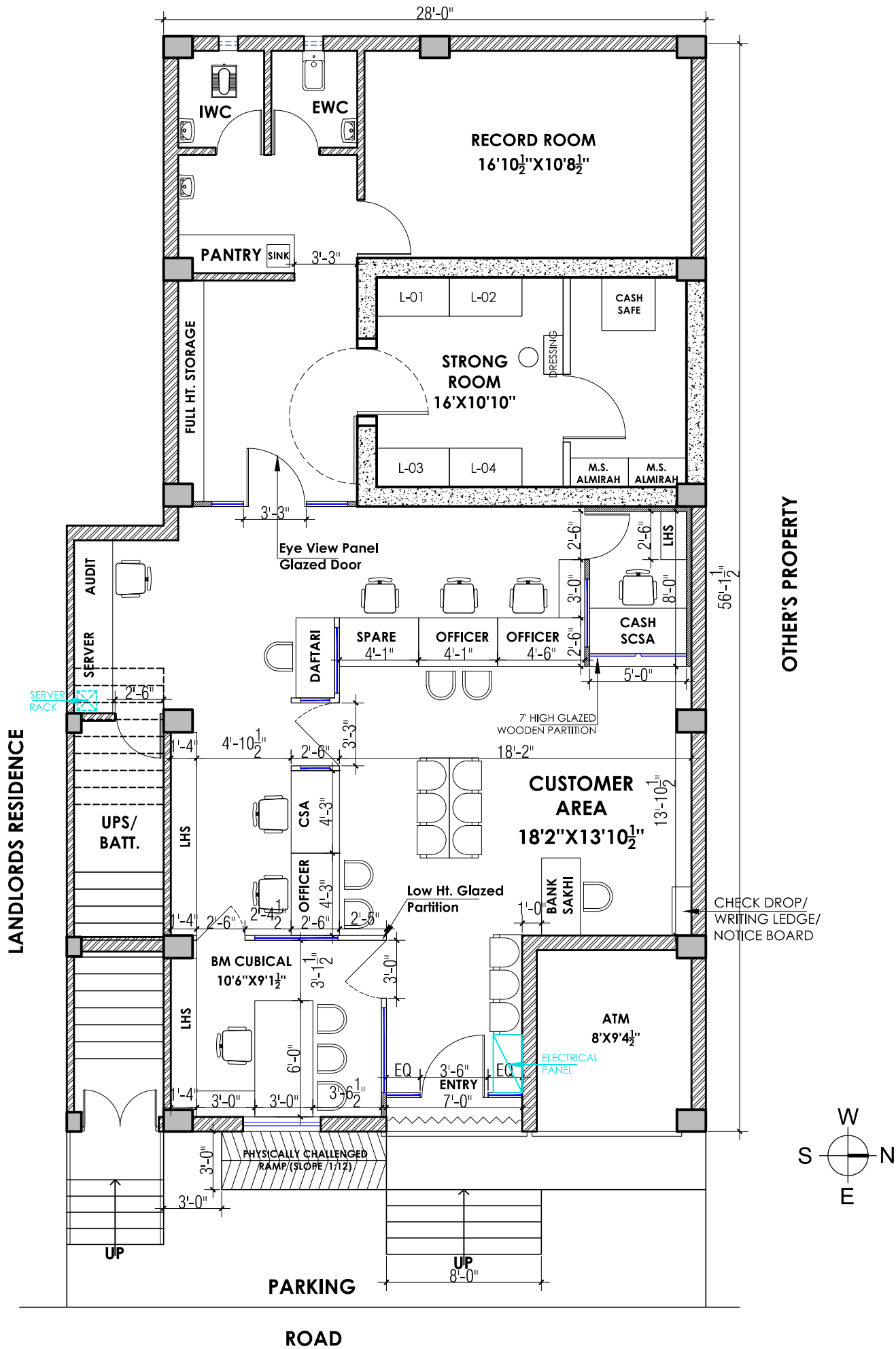
FURNITURE LAYOUT PLAN BO KANNAUJ
