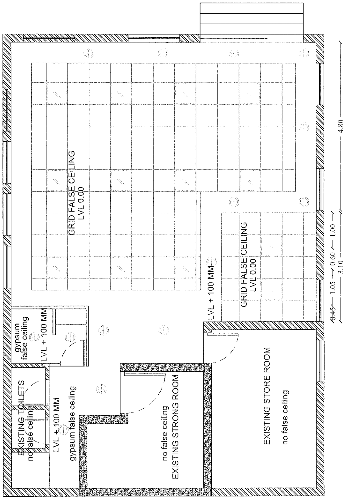
RAVER BRANCH RO JALGAON FALSE CEILING LAYOUT
